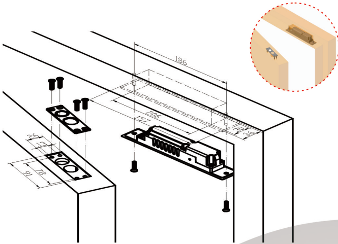
Installation on top for solid door
