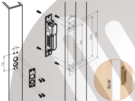
Side installation for hollow door
