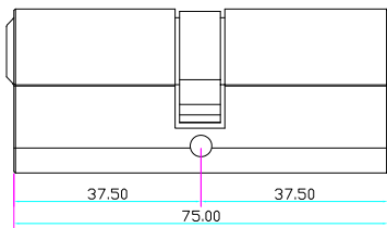
Double side cylinder
