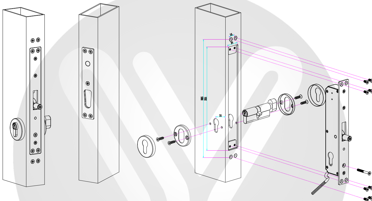
Side installation for hollow door
