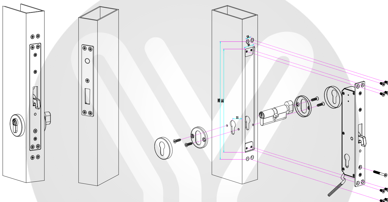
Side installation for hollow door
