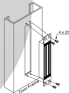
(4) Fix screws
